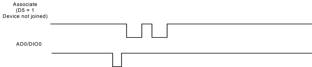
A single commissioning button press when the device has not joined a network that causes the associate pin to blink to indicate the AI Code where: AI = # blinks + 0x20. In this example, AI = 0x22.
