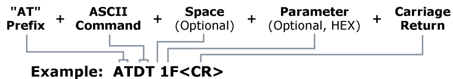
Figure 2: Syntax for sending AT commands
